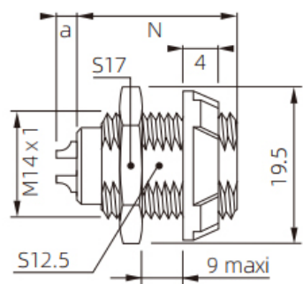
焊接+压接 (Solder + Crimp)
