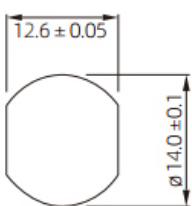
开孔尺寸 (Hole opening size)
